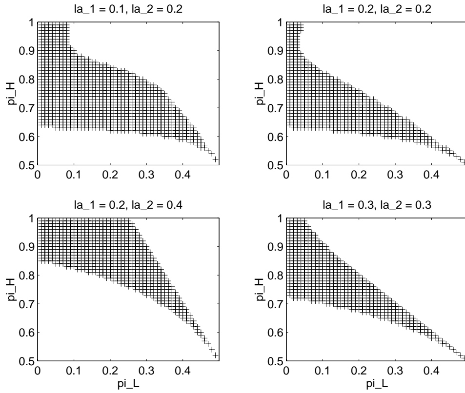
Figure 2: Shaded area shows the [\pi_L, \pi_H] pairs which satisfy the sufficient conditions for both underreaction and overreaction for a variety of different values of \lambda_1 and \lambda_2 . \pi_L ( \pi_H ) is the probability, in the mean-reverting (trending) regime, that next period's earnings shock will be of the same sign as last period's earnings shock. \lambda_1 and \lambda_2 govern the transition probabilities between regimes.
