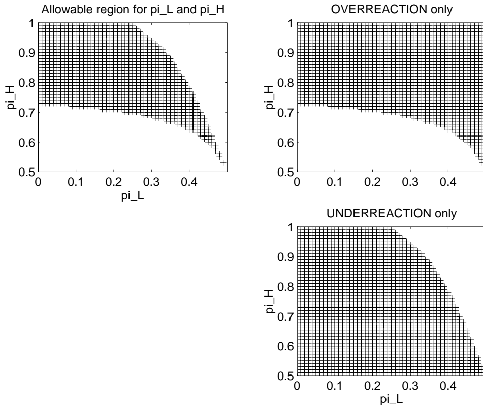
Figure 1: Shaded area in graph at top left marks the [\pi_L, \pi_H] pairs which satisfy the sufficient conditions for both underreaction and overreaction, when \lambda_1 = 0.1 and \lambda_2 = 0.3 . Graph at top right (bottom right) shows the [\pi_L, \pi_H] pairs that satisfy the condition for overreaction (underreaction) only. \pi_L ( \pi_H ) is the probability, in the mean-reverting (trending) regime, that next period's earnings shock will be of the same sign as last period's earnings shock. \lambda_1 and \lambda_2 govern the transition probabilities between regimes.
